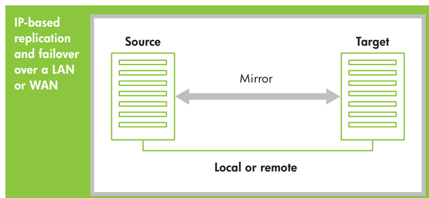
Figure 1: Simple one-to-one HP Storage Mirroring replication and failover configuration.
